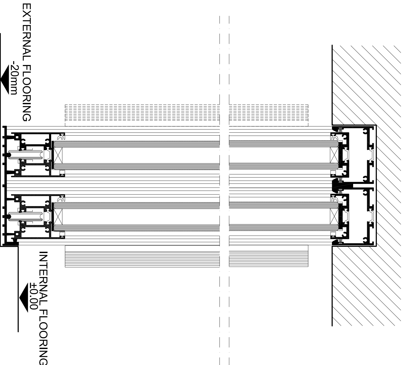
VERTICAL SECTION
